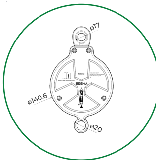
POLEA PRINCIPAL
